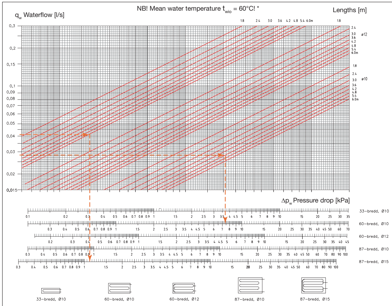
Diagram 4. Panels, pressure drop at 60^\circ\text{C} . For pressure drops at temperatures other than 60^\circ\text{C} , the pressure drop is multiplied by the pressure drop factor (see diagram 7).
