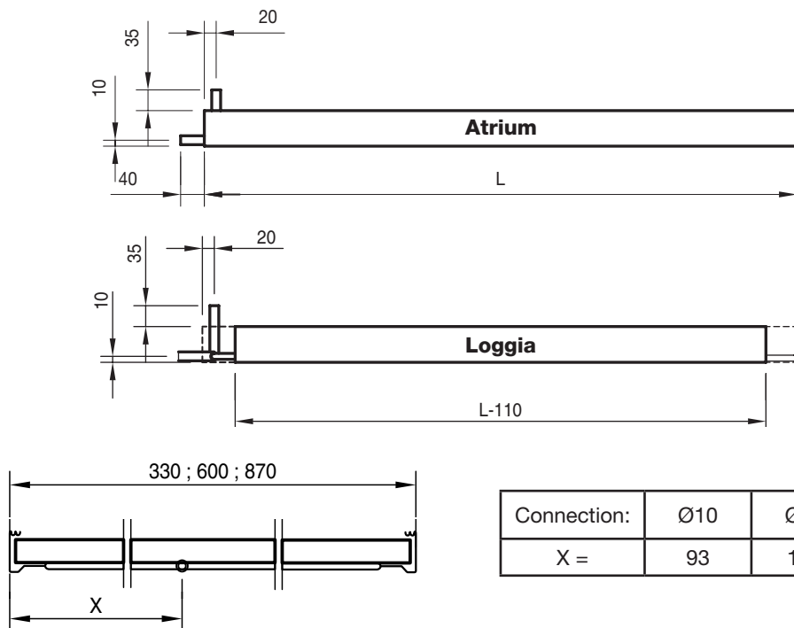
Figure 4.b. Atrium and Loggia dimension, water connection and connection.
